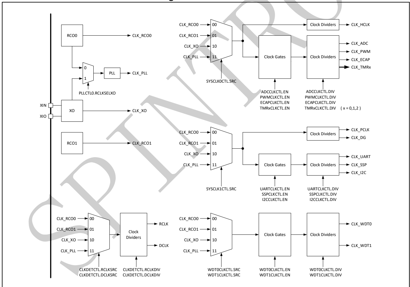
Figure 2-1: Clock tree
