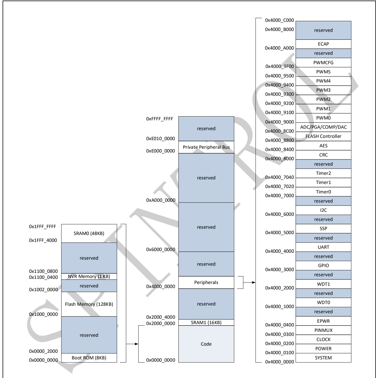
Figure 4-1: Memory map
